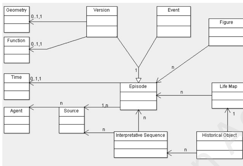
FIGURE 3: IMPROVED CORE DATA MODEL.
