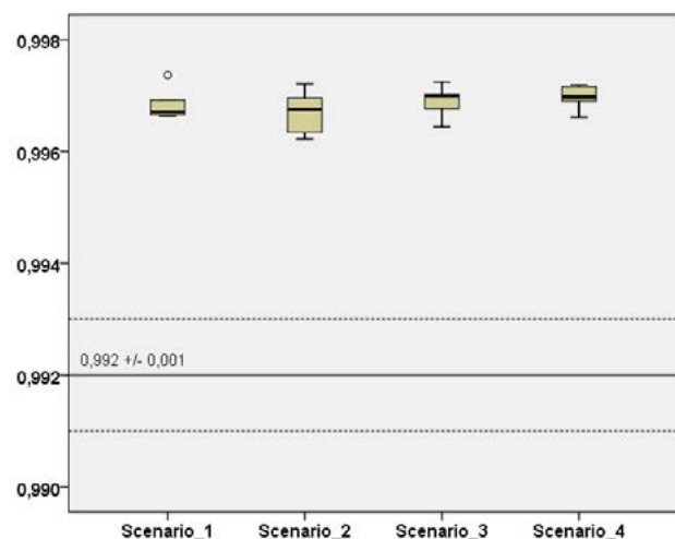
FIGURE 3: THE Y-STR HAPLOTYPEDIVERSITY ( \hat{H} ) IN FINAL POPULATION (0 BP) WITH SCENARIOS 1-4 WITH 50 SIMULATION REPLICATES, EACH WITH A SAMPLE OF 907 INDIVIDUALS. THE REFERENCE LINE REPRESENTS THE VALUE OBSERVED IN THE PRESENT ( 0.992 \pm 0.001 ) (PALO ET AL. 2009). THE NUMBER OF INDIVIDUALS IN A SAMPLE CORRESPONDS TO THE SAMPLE SIZE IN PALO ET AL. 2009 ENABLING DIRECT COMPARISON BETWEEN THE SIMULATIONS AND THE REAL WORLD.
