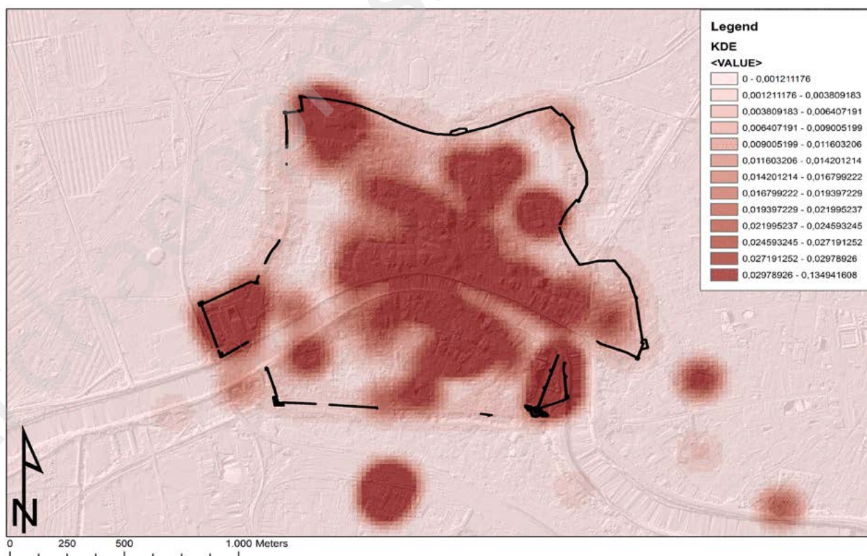
FIGURE 6: THE KDE PREDICTIVE TEST VISUALISED AS A ¼ STANDARD DEVIATION. THE RESULT OBTAINED IS AN APPROXIMATE IDEA OF THE DATA SPATIAL STRUCTURE, I.E. OF THE CONCENTRATION OF LATE MEDIEVAL ARCHAEOLOGICAL FINDINGS, BUT, PRACTICALLY, ITS NON-PARAMETRIC FUNCTION DEPICT A SORT OF SELF-FULFILLING PROPHECY.
