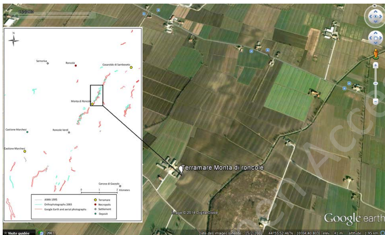
FIGURE 8: TRACE OF PALEOCHANNEL, SUPPOSED TO HAVE BEEN ACTIVE DURING THE BRONZE AGE, IN RELATIONSHIP WITH THE TERRAMARE SITE OF MONTA DI RONCOLE (GOOGLE EARTH V 7.1.2.2041. (15 FEBRUARY 2003). MONTA DI RONCOLE, ITALIE. 44°55'52.46'N, 10°04'40.80'E, ALTITUDE: 1, 95 KILOMETER. DIGITALGLOBE 2014).
