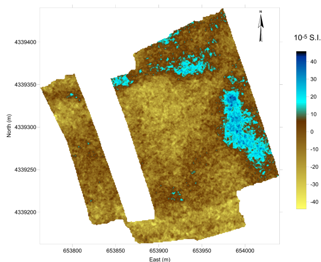
FIGURE 13: APPARENT MAGNETIC SUSCEPTIBILITY MAP AT ALMIRIOTIKI SITE, THESSALY (GREECE) (GEM-2, HCP)
