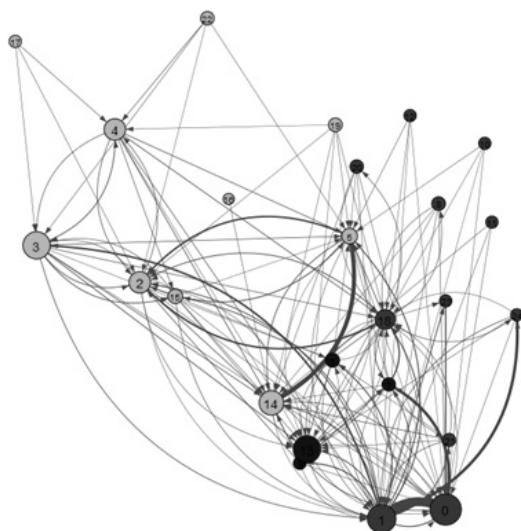
FIGURE 5: COMMUNITIES AND INTERACTIONS FROM ARIADNE MODEL (100KM) NETWORK. EACH SITE IS REPRESENTED AT A CIRCLE (AND NUMBERED ACCORDING TO TABLE 1), WHERE THE SIZE DENOTES ITS ESTIMATES INPUT SIZE AND THE COLOUR SIGNIFIES IT COMMUNITY AFFILIATION BASED ON ITS INTERACTIONS. THE INTERACTIONS ARE REPRESENTED BY THE EDGES INCREASE IN SIZE IN PROPORTION TO THE MAGNITUDE OF INTERACTION ON THE EDGES. THE ARROWS DENOTE THE DIRECTION OF THE INTERACTION.
