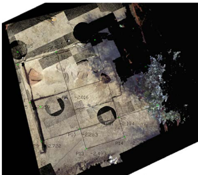
FIGURE 10: 2D ORTHOIMAGE.
