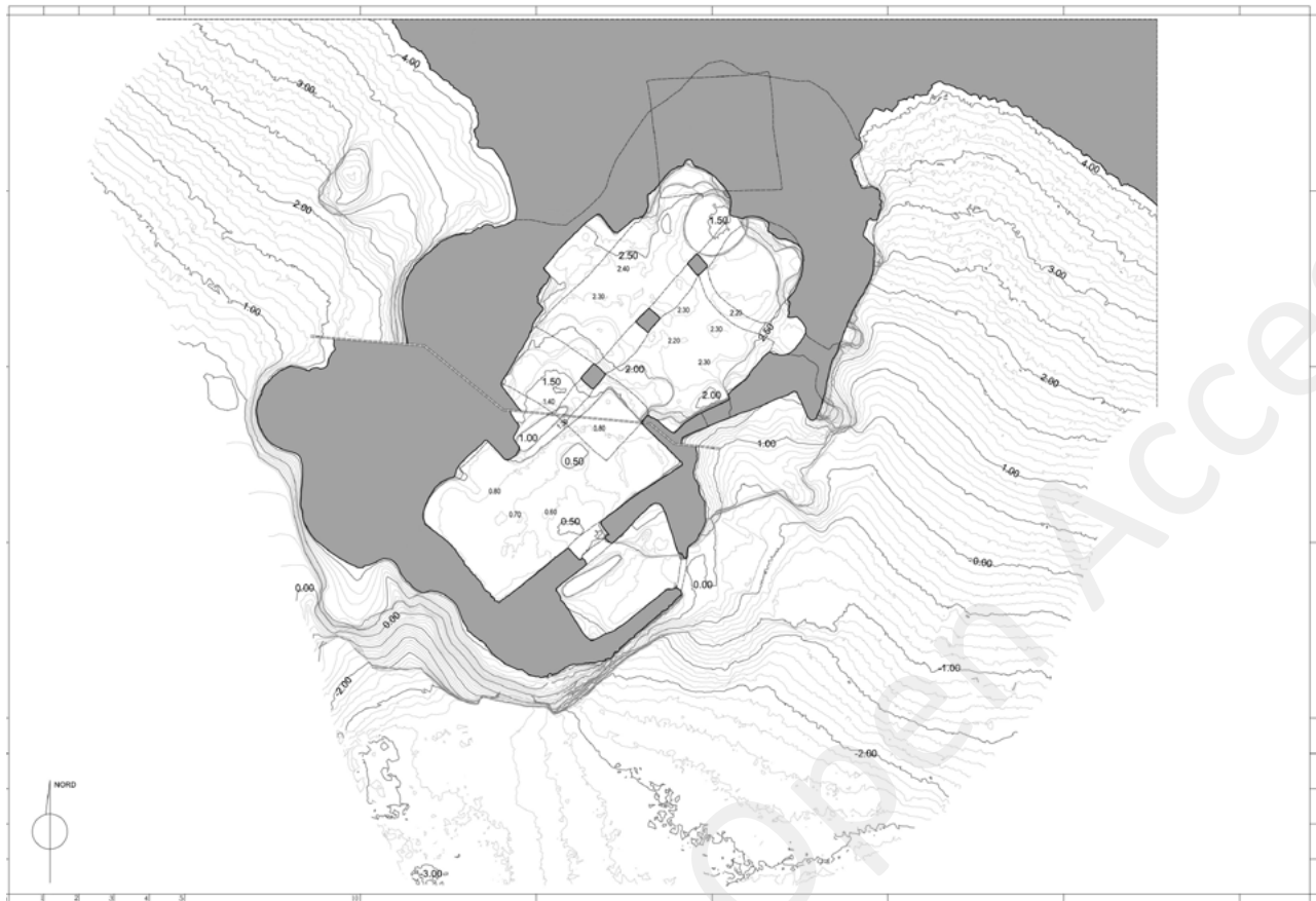
FIGURE 8: TURKEY, CAPPADOCIA, SAHINEFENDI, CHURCH OF THE FORTY MARTYRS, PLANT OF THE ENTRANCE LEVEL AND THE CHURCH, CONTOUR LINES AT 10CM EQUIDISTANT.
