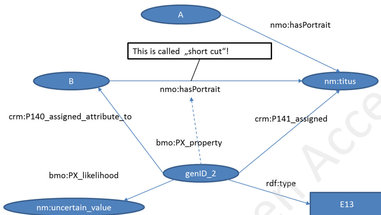
FIGURE 6: USING CIDOC CRM/RS IN ORDER TO EXPRESS THAT FOR COIN B IT IS UNCERTAIN IF IT HAS A PORTRAIT OF TITUS, WHILE FOR COIN A THIS IS CERTAIN.
