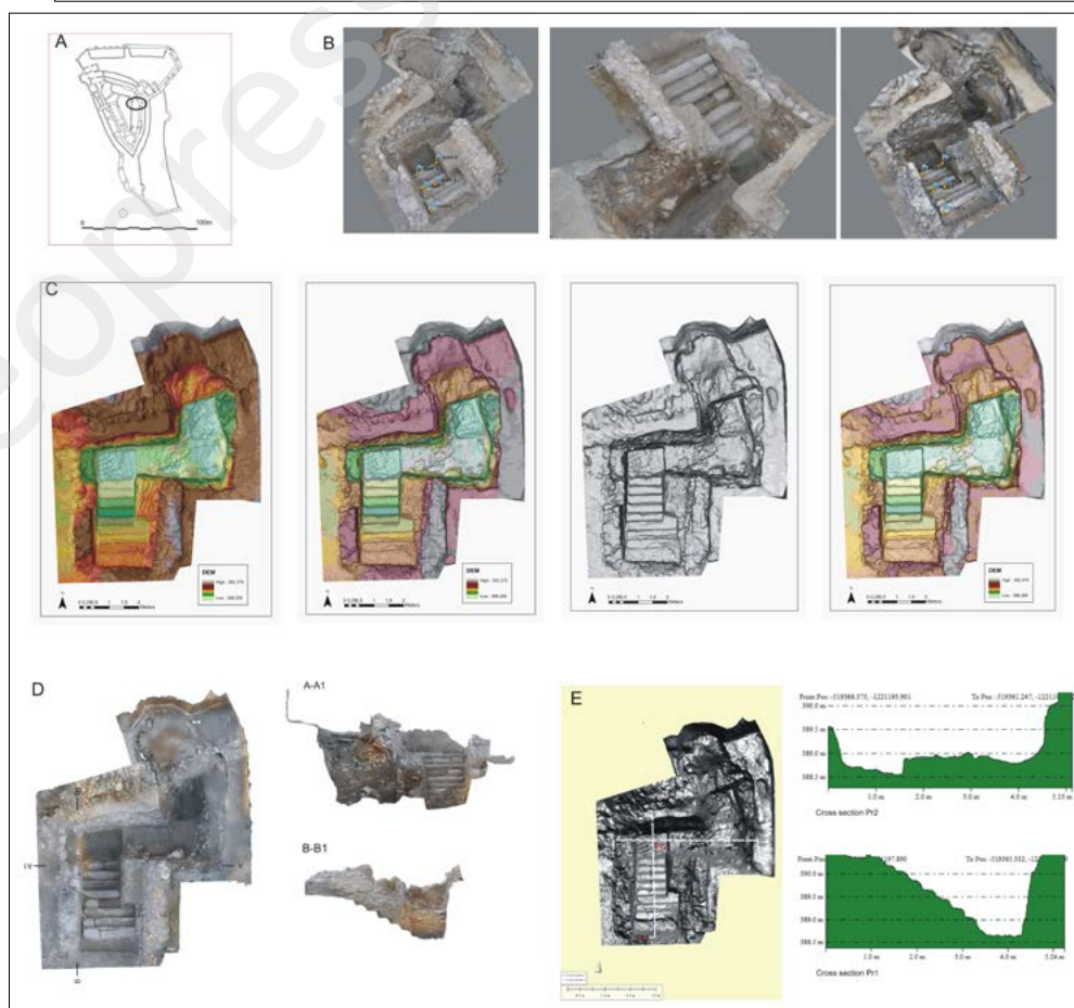
FIGURE 9: THE ČAČTICE CASTLE. TRENCH S3 IN EASTERN PALACE. A-LOCATION OF THE TRENCH WITHIN THE CASTLE LAYOUT, B-SOLID 3D MODEL OF THE TRENCH WITH TEXTURE MAP, C- DEM WITH DIFFERENT FORMS OF VISUALISATION (ANALYTICAL HILLSHADING AND HYPSONETRY), D- ORTOPHOTOPLAN OF THE LAYOUT AND PROFILES, E- CROSS SECTIONS. PHOTOS: 28 (HAND HANDLED CAMERA). MESH: 1,1 MILLIONS FACES.
