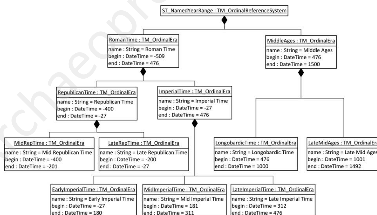
FIGURE 4: EXAMPLES OF ORDINAL ERAS USED IN SITA*R.
