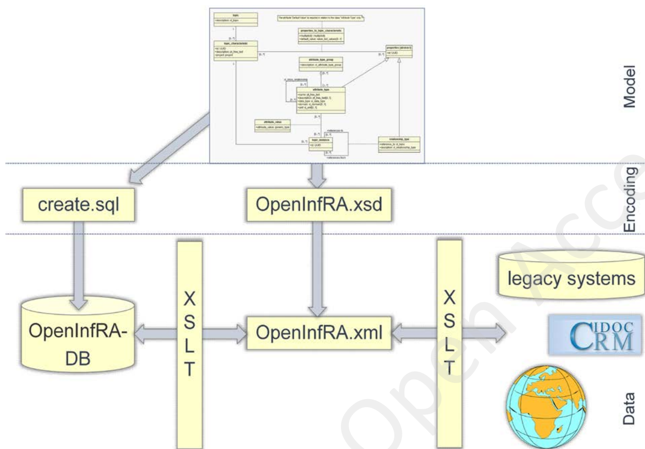
FIGURE 7: OPENINFRA XML INTERFACES.
