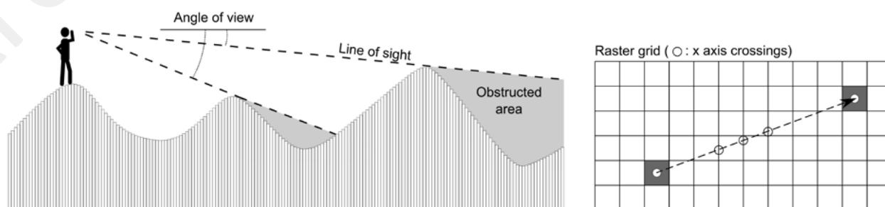
FIGURE 2: INTERVISIBILITY CALCULATION.
