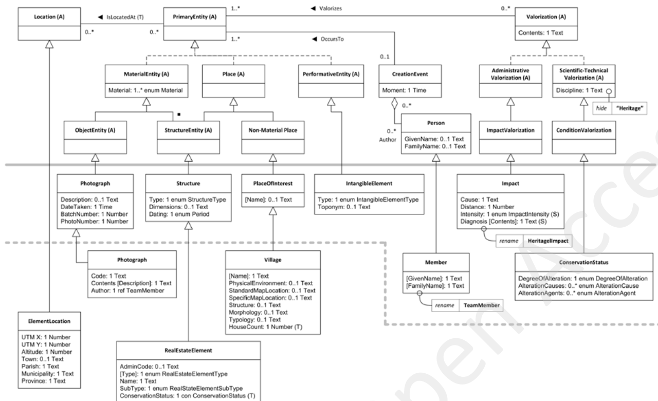
FIGURE 9: PARTICULAR MODEL FOR CAMINHO EXPRESSED IN TERMS OF THE INCIPIT CSIC SHARED MODEL. CLASSES ABOVE THE SOLID GREY LINE ARE PART OF CHARM. CLASSES BELOW THE SOLID GREY LINE AND ABOVE THE DOTTED GREY LINE HAVE BEEN ADDED TO CAPTURE CONCEPTS SPECIFIC TO INCIPIT CSIC AS DETERMINED BY COMMONALITIES TO BOTH SIA AND CAMINHO (SEE FIGURE 7). CLASSES BELOW THE DOTTED GREY LINE HAVE BEEN ADDED TO CAPTURE CONCEPTS SPECIFIC TO CAMINHO.
