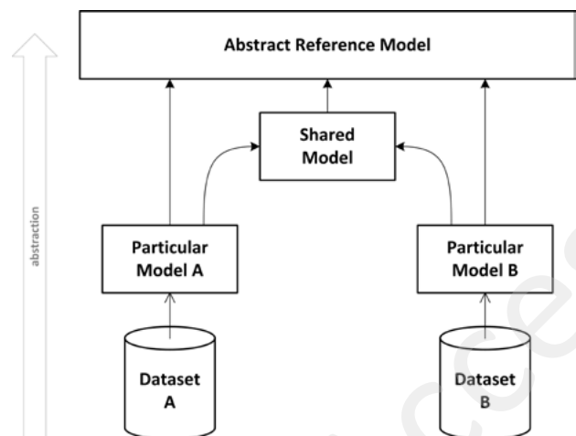
FIGURE 2: OVERALL ARCHITECTURE OF THE PROPOSED SOLUTION. DATASETS ARE DEPICTED AS CYLINDERS AND MODELS AS RECTANGLES. STICK ARROWHEADS DEPICT DATA CONFORMANCE TO A MODEL, AND FILLED IN ARROWHEADS DEPICT CONFORMANCE BETWEEN MODELS. ABSTRACTION INCREASES FROM BOTTOM TO TOP.
