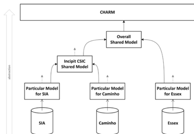
FIGURE 3: HYPOTHETICAL ARCHITECTURE FOR THE CASE STUDY. LIKE IN FIGURE 2, DATASETS ARE DEPICTED AS CYLINDERS, MODELS ARE DEPICTED AS RECTANGLES, STICK ARROWHEADS DEPICT DATA CONFORMANCE TO A MODEL, AND FILLED IN ARROWHEADS DEPICT CONFORMANCE BETWEEN MODELS. INDIRECT CONFORMANCE BETWEEN MODELS (I.E. THAT WHICH IS A RESULT OF LISKOV SUBSTITUTABILITY) IS SHOWN AS GREY DASHED ARROWS FOR CLARITY.
