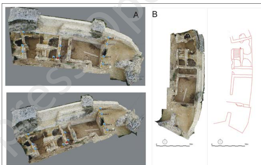
FIGURE 11: THE ČACHTICE CASTLE. EASTERN PALACE. A-SOLID 3D MODEL WITH TEXTURE MAP, B-VECTORISED ORTOPHOTOPLAN. PHOTOS: 45 (UNMANNED AERIAL VEHICLE). MESH: 1,7 MILLIONS FACES.
